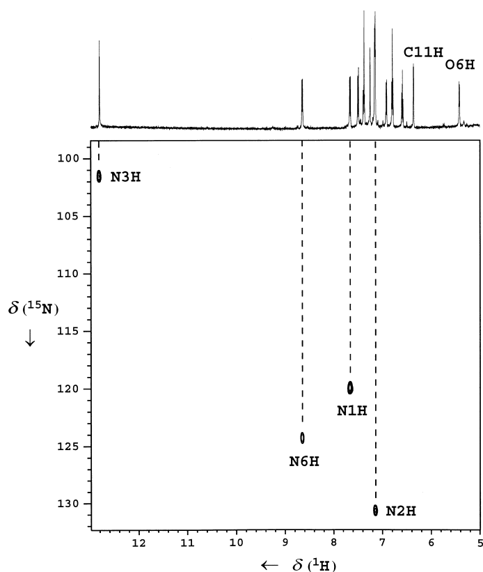
Figure 2. Partial ^1\text{H}/^{15}\text{N} -HSQC spectrum (500 MHz, [\text{D}_6] DMSO) of natural diazonamide A.
