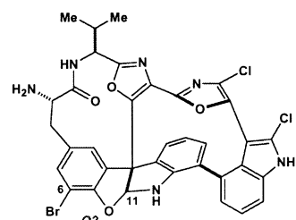
5 (–)-diazonamide B (revised Structure)
